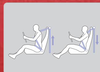
Pretensioner seat belts with load limiter
